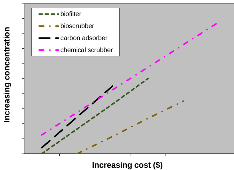
Figure 6: Chart comparing the treatment costs versus H 2 S concentration for the various treatment types.
