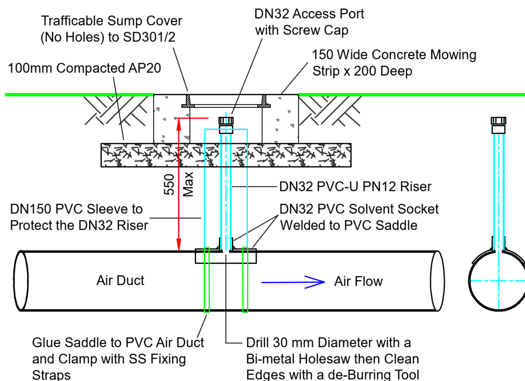
Figure 9: Example Factory Made access port for air velocity and air flow rate measurement.
