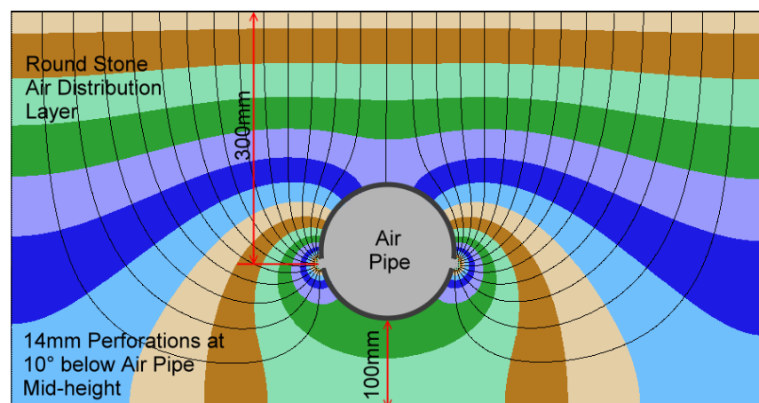
Figure 8: Plenum air flow pattern for DN150 air pipes at 900 centres and 14mm diameter perforations at 300mm below the plenum top surface.
