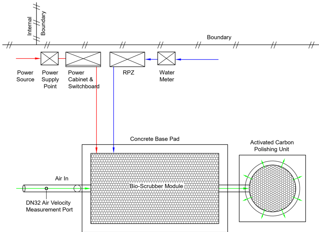
Figure 14: Typical Bio-scrubber Site Layout. Note that the power box and switchboard cabinet should generally be against the boundary and adjacent to the internal common boundary.
