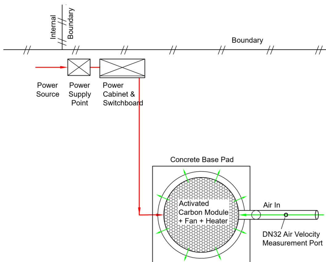
Figure 12: Typical Activated Carbon Site Layout. Note that the power box and switchboard cabinet should generally be against the boundary and adjacent to the internal common boundary.
