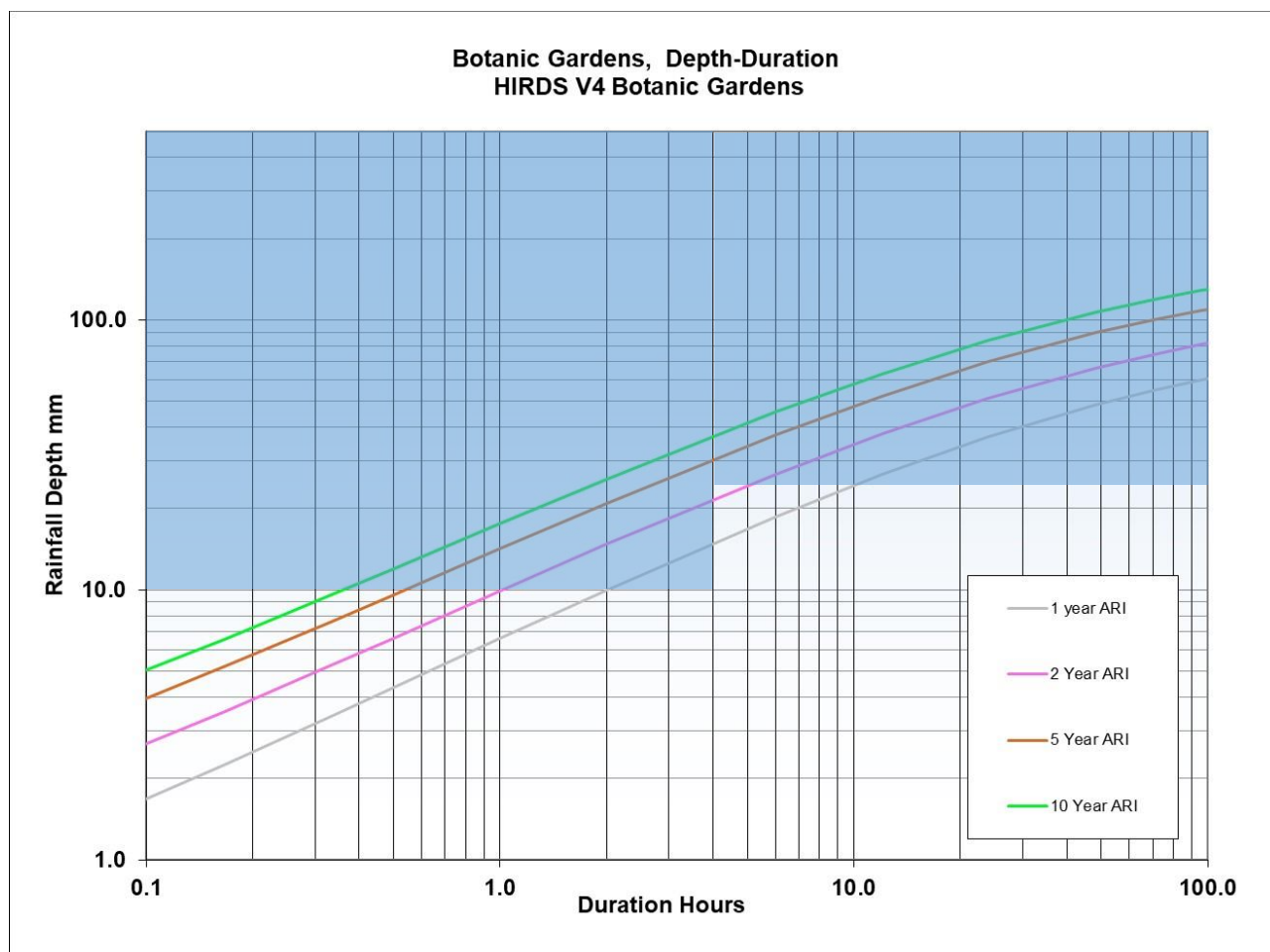
Figure 3 Botanic Gardens – Depth-Duration frequency from HIRDS v4
